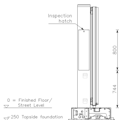
Cross Section J-J
